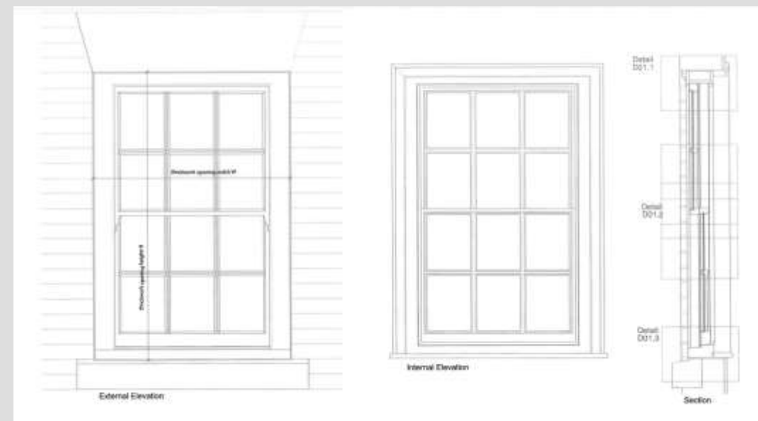
Figure 43: Box sash window example
